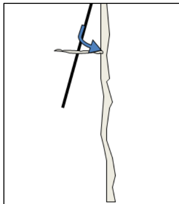
Figure 4. Illustration of indirect grouting connection of large fracture from a tight fracture.
